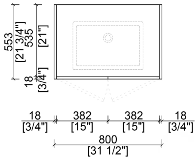
BASE CABINET PLAN
