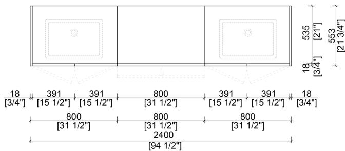
FRONT ELEVATION
