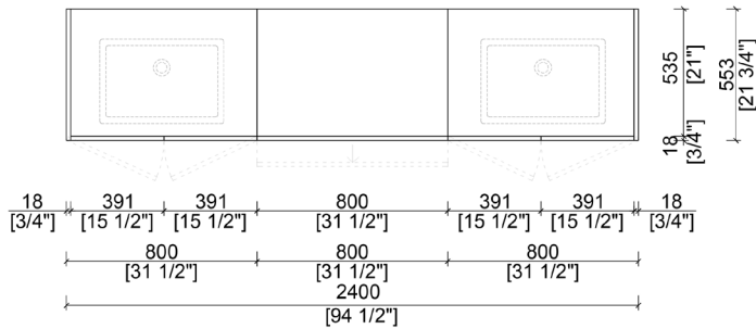
FRONT ELEVATION
